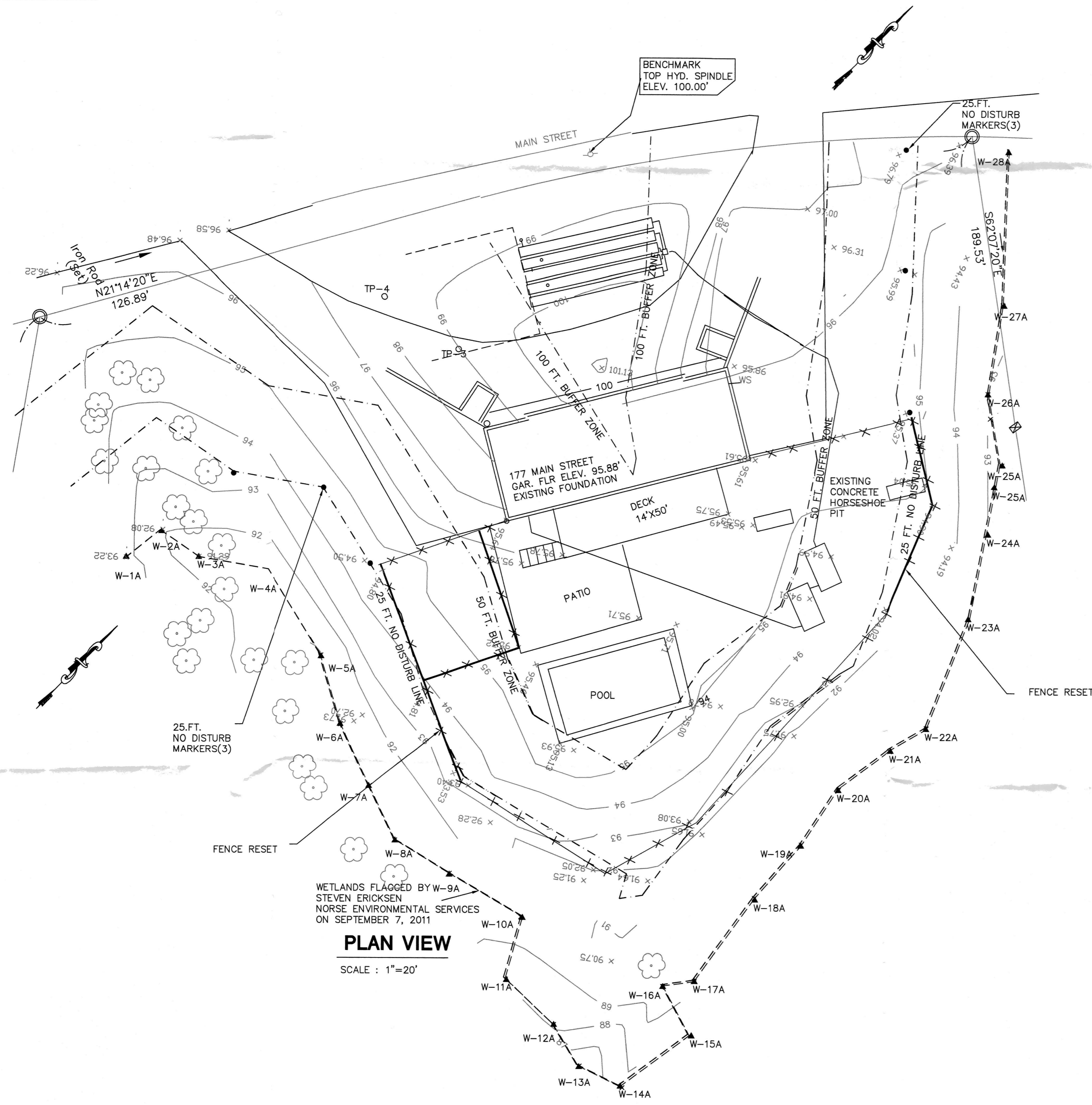
EXISTING AND PROPOSED REMEDIATION WORK SCALE : 1"=20'
