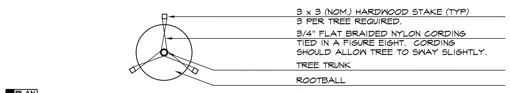
PLAN
