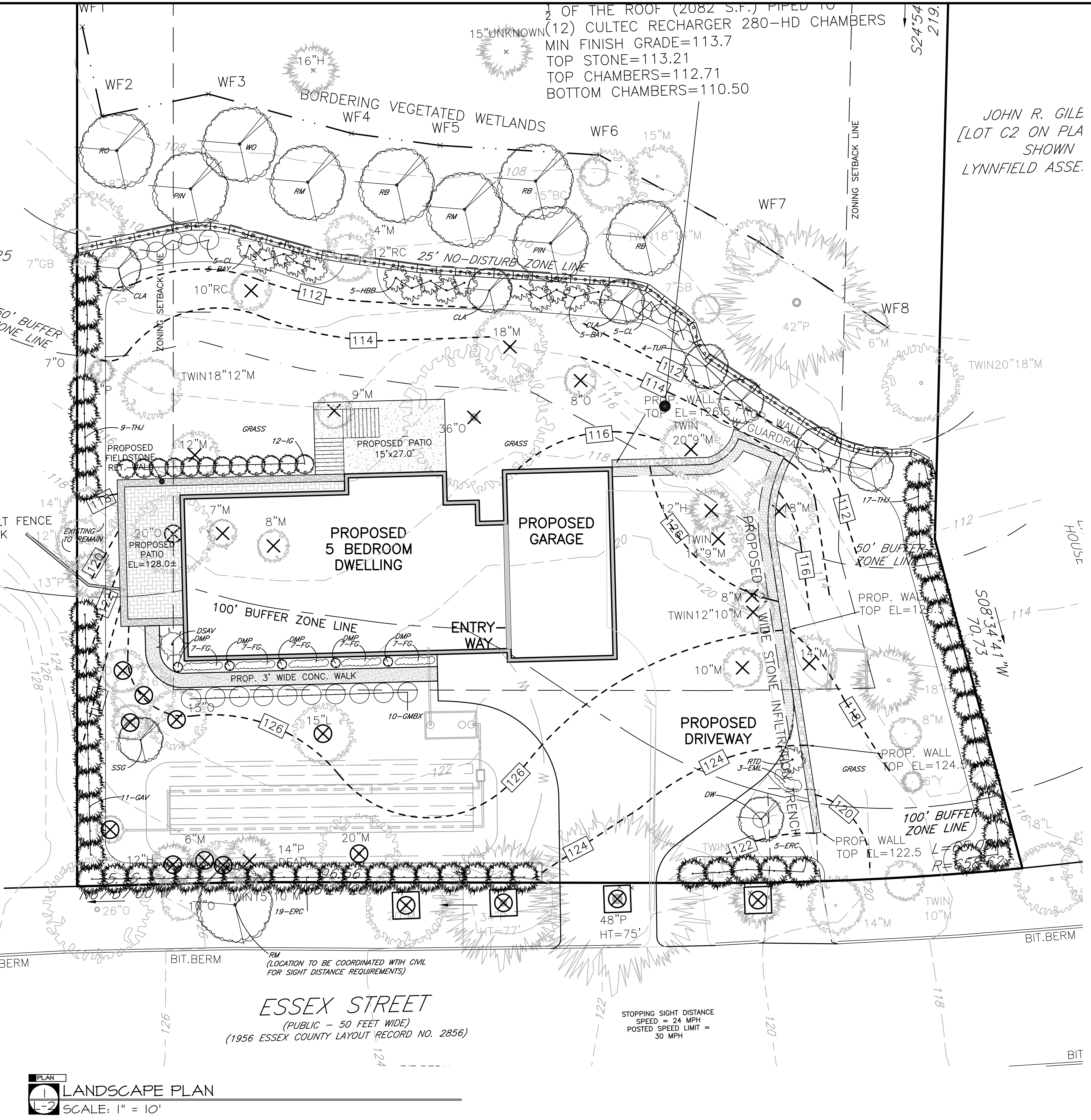
PLAN
