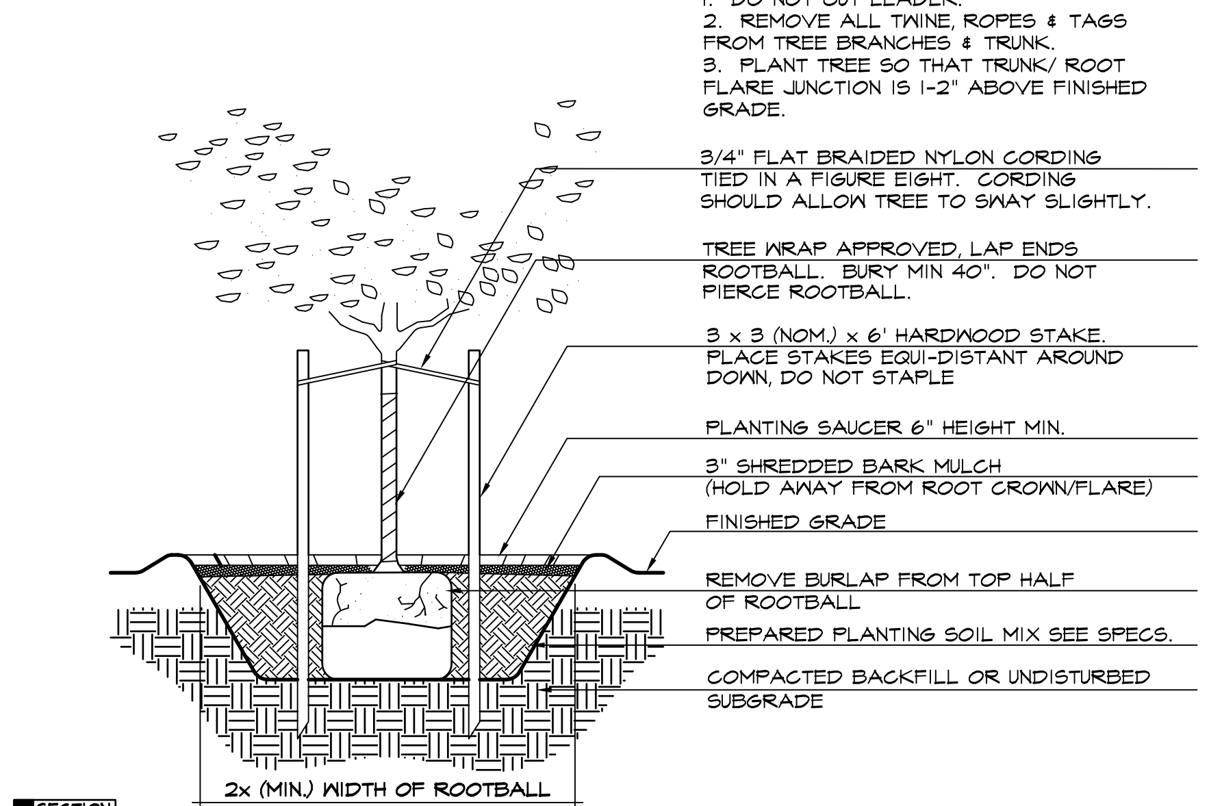
SECTION
