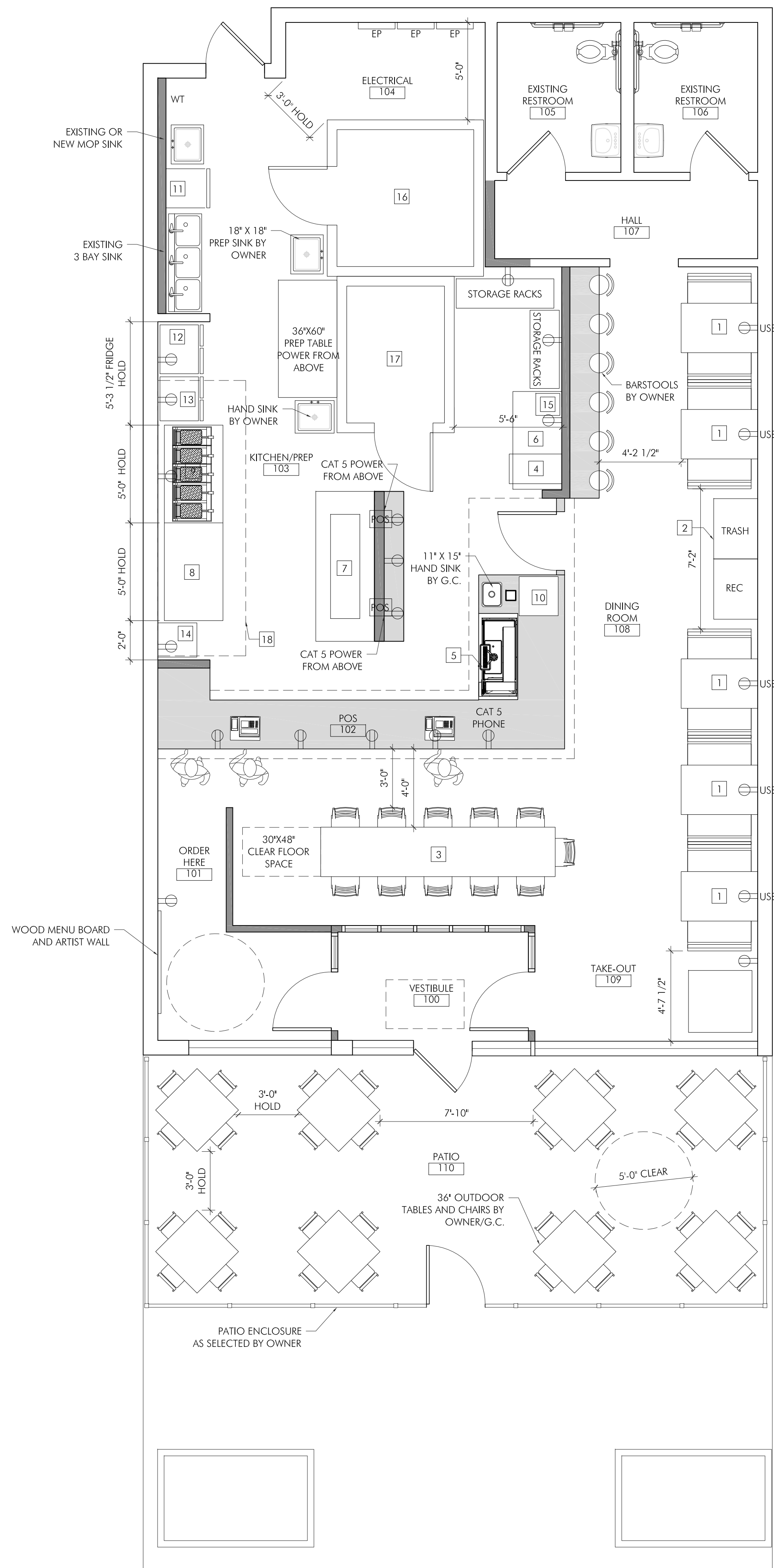
FURNITURE & EQUIPMENT/POWER PLAN SCALE: 1/4" = 1'-0"
